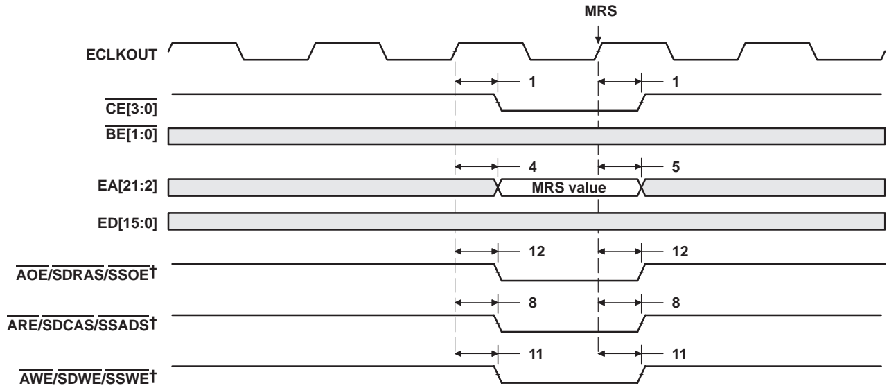
Figure 36. SDRAM MRS Command
